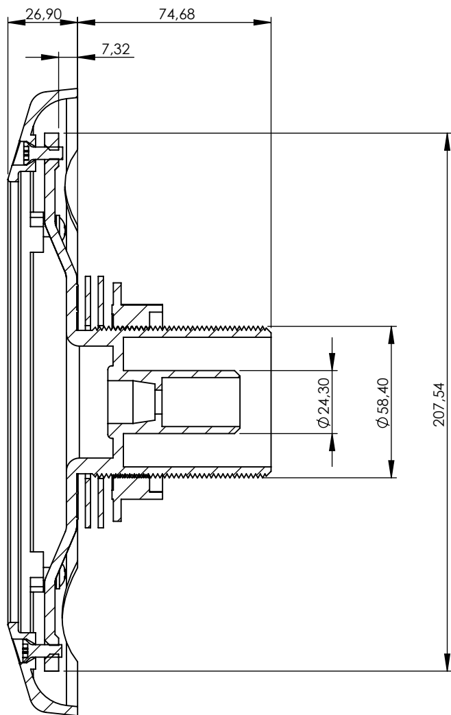
SECTION F-F
