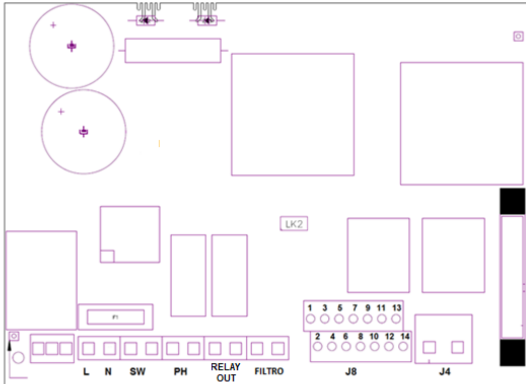
Power Board
