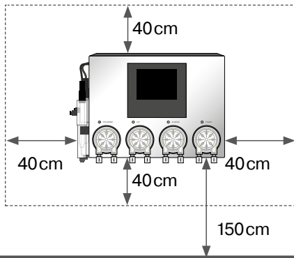
Wall bracket
